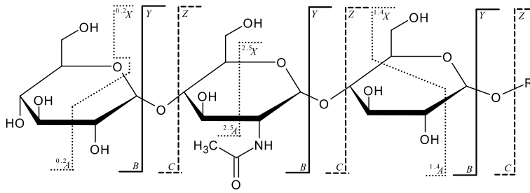
Figure 11.3: Fragments resulting from tandem mass spectrometry analysis of a glycan. Note that B, C, Y, and Z ions are not affected by linkage types.
