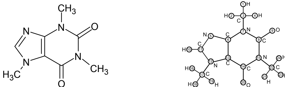
Figure 10.1: Left: Structural formula of caffeine, molecular formula C_8H_{10}N_4O_2 , monoisotopic mass 194.080376 Da. Right: Corresponding molecular graph with colors from \{C, H, N, O\} , but without bond orders. Note that some hydrogen atoms are omitted in the structural formula.
