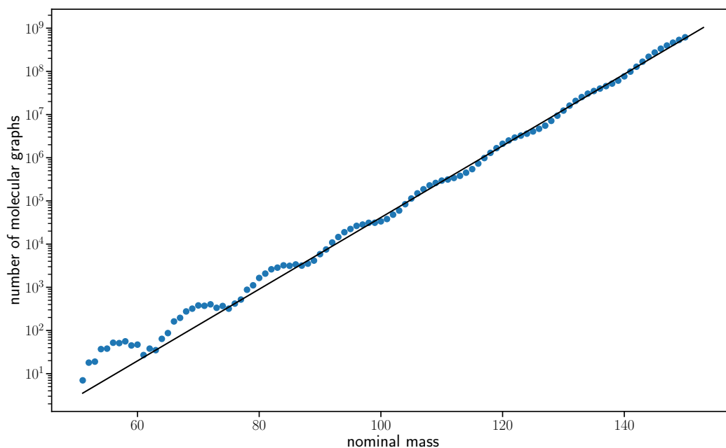
Figure 10.3: Number of molecular graphs with nominal mass m . Numbers taken from Kerber et al. [153]. Note the logarithmic y-axis. Regression line fitted for masses 80 Da and above.
