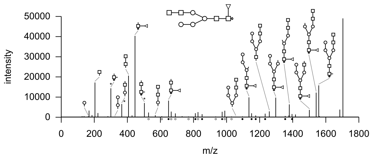
Figure 11.4: The peak-picked spectrum of a glycan with four hexoses, four N-acetylhexosamines, and one fucose. The spectrum is annotated with single-cleaved fragments of the correct glycan topology, and all but one peaks corresponding to single-cleaved fragments are found in the spectrum. Three intense peaks marked with (*) correspond to double-cleaved fragments. Additionally, all peaks marked with filled circles can be annotated with double-cleaved fragments of the glycan, and peaks marked with unfilled circles can be annotated with fragments that stem from more than two cleavages. Figure from [32].
